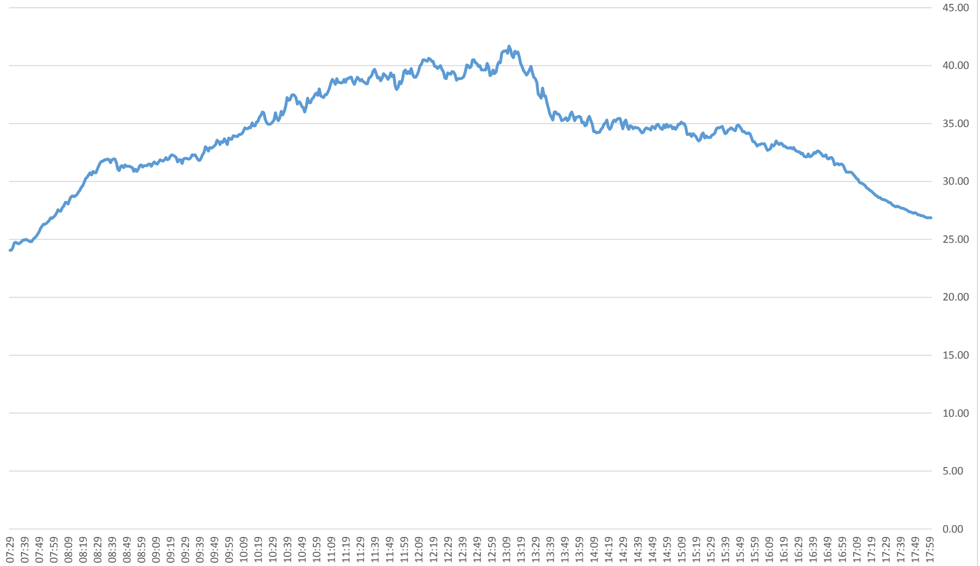
Temperature (C) - Goiania/Goias - 20/05/16
